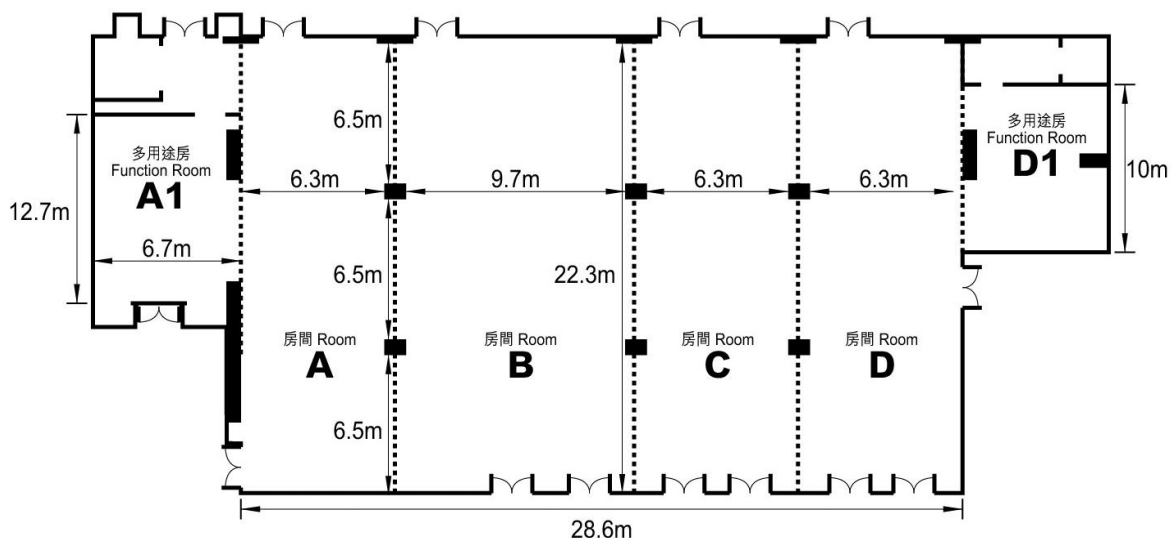
宴會廳 - 平面圖 (700平方米) Grand Ballroom - Floor Plan (700m 2 )
